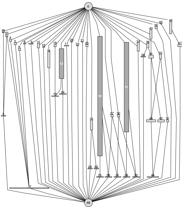
Figure 3: The lattice of aspect candidates from a commit to Eclipse CVS on 2004-02-25 by developer pttf. Candidate 10, e.g., contains 104 additions of calls to preReplaceChild(3) , postReplaceChild(3) .
