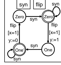
Figure 13. The Modulo2Counter component.
