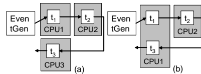
Figure 8. End to end delay measurement for tasks.
