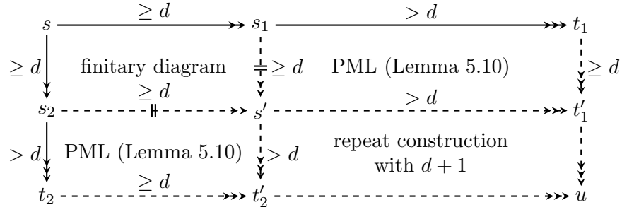
Figure 8: Infinitary confluence.
