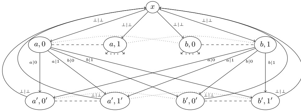
■ Figure 1 A distributed game \mathcal{G}_{\parallel} .
