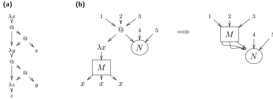
■ Figure 3 (a) A dag-representation of \lambda x. (\lambda y. (\lambda z. z) ((\lambda z. z) y)) ((\lambda y. (\lambda z. z) ((\lambda z. z) y)) x) . (b) A graph rewriting rule corresponding to (\lambda x. M)N \rightarrow M[N/x] .
