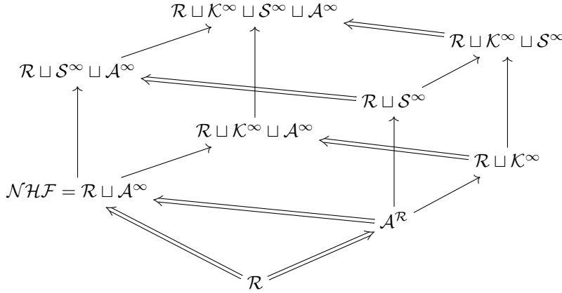
■ Figure 1 A fragment of \mathcal{L}_{CL} : single (double) arrows indicate that the corresponding open intervals are singletons (uncountable). A similar fragment can be built by replacing \mathcal{R} by \mathcal{H} in the above diagram.
