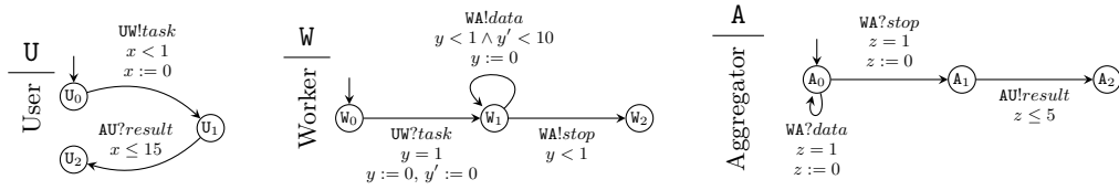
■ Figure 1 Scheduled Task Protocol (System S_{ST} ).
