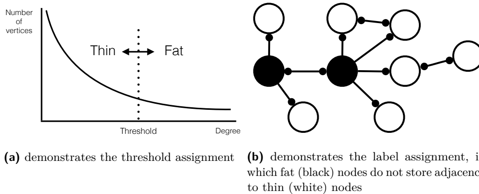
■ Figure 1 Two illustrations of the main idea.
