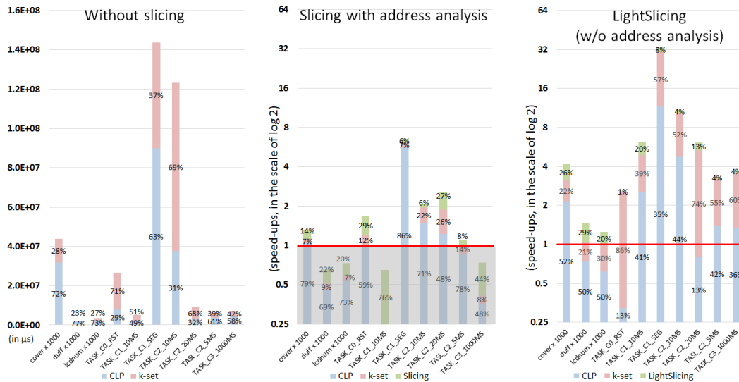
Figure 2 Execution comparisons of the dynamic branching analyses.
