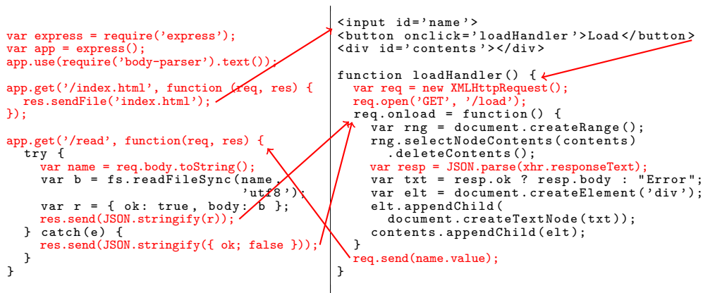
■ Figure 1 A canonical two-tier web application.
