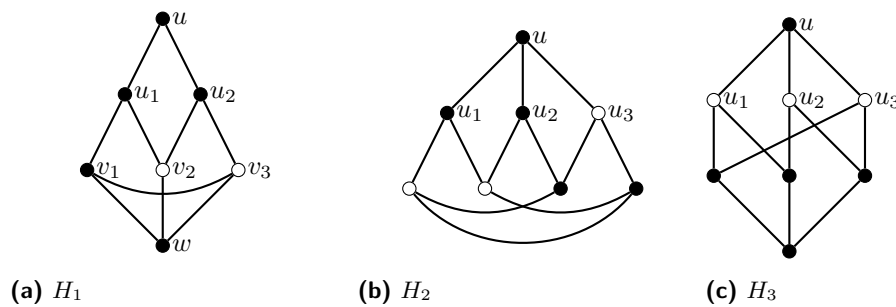
■ Figure 2 The graphs used in Rule 8. A near-bipartite decomposition of each is indicated: the white vertices form an independent set and the black vertices induce a forest.
