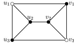
(b) triangular prism
