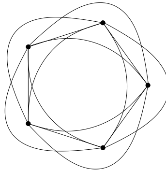
■ Figure 1 Theorem 5 is tight for every n \geq 3 . Construction for n = 5 .
