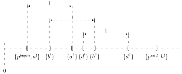
■ Figure 5 A trace encoding the halting computation of the DCM in Figure 4. Note that each m^i is followed by a corresponding m^{i+1} exactly 1 time unit later.
