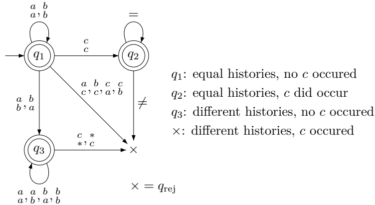
Figure 2 A two-tape DFA defining an indistinguishability relation that does not correspond to any regular observation function (the symbol = stands for \{a, b, c\} , the symbol \neq stands for \{x \in \Gamma \times \Gamma \mid x \neq y\} , and the symbol * stands for \{a, b, c\} ).
