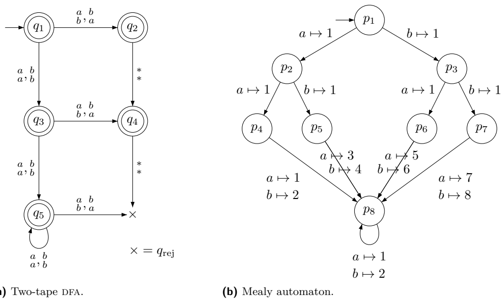
Figure 3 A synchronous two-tape automaton with 2k states (here k = 3 ) for which an equivalent observation Mealy automaton requires exponential number of states ( 2^k ).
