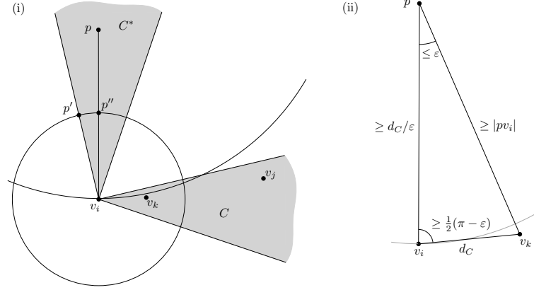
■ Figure 7 Illustration for Case III.
