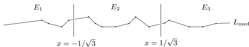
■ Figure 5 The edge sets E_1, E_2 , and E_3 of L_{\text{med}} , the median level in \mathcal{A}(V^*) .
