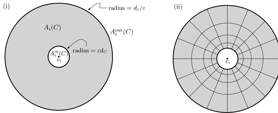
■ Figure 6 (i) The closed spherical shell A_i(C) defined by the two balls of radii \epsilon \cdot d_C and d_C/\epsilon around v_i . (ii) The exponential grid G_i(C) . The grid is defined by a collection of spheres centered at v_i , plus extreme rays of the cones with apex at v_i . The spheres have radii (1 + \epsilon/4)^i \cdot \epsilon \cdot d_C for 0 \leq i \leq \log_{(1+\epsilon/4)}(1/\epsilon^2) = O((1/\epsilon) \log(1/\epsilon)) , and the interior angle of a cone is \epsilon/2\sqrt{d} .
