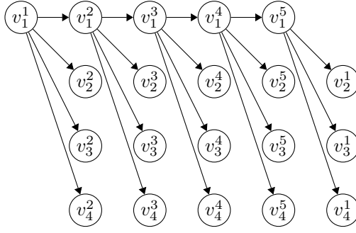
■ Figure 1 The spanning tree construction for width 4 and d = 5 .
