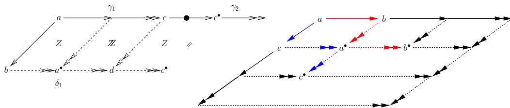
Figure 5 Hyper-cofinality of \twoheadrightarrow (left) and confluence of \rightarrow (right), by tiling with Zs.
