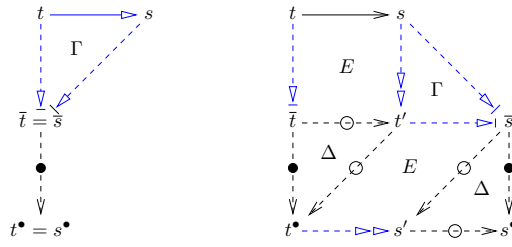
Figure 4 \lambda\sigma has the Z-property.
