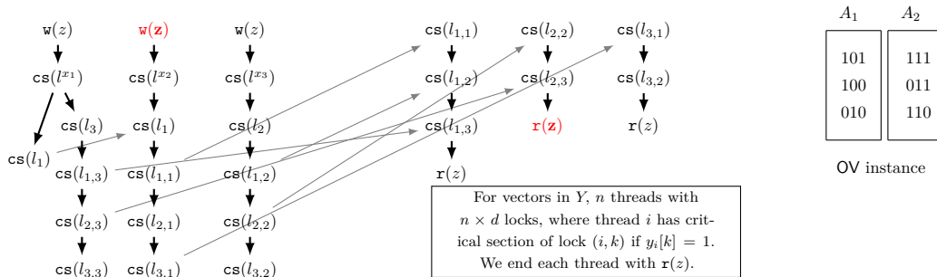
■ Figure 2 Reducing OV to finding HB races. For simplicity, we show the graph G_{\text{HB}}^\sigma instead of the trace \sigma . The HB race is marked in red, corresponding to the orthogonal pair (x_2, y_2) .
