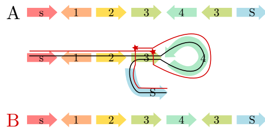
■ Figure 1 Illustration of an NAHR-mediated inversion. Haplotype A (black line) represents the original configuration, while haplotype B (red line) can be derived from A by two recombination events between inverted repeats of genomic marker 3 as indicated by the red stars.
