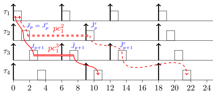
Figure 4 Four tasks with cause-effect chain (\tau_1 \rightarrow \tau_2 \rightarrow \tau_3 \rightarrow \tau_4) communicating via implicit communication. The red line depicts the chain pc_1^3 whereas the dashed red line depicts pc_1^2 . The length of pc_1^3 is upper bounded by the length of pc_1^2 . The blue job annotations illustrate the proof of Lemma 12 ( \geq -relation).
