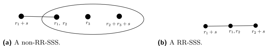
■ Figure 1 Access structure 1a contains a minimal set of size 2 and a minimal set of size 3. Access structure 1b contains two minimal sets of size 2. The secret is a single bit s and r_i s are the randomness. The value written under each party, indicates that party's share.
