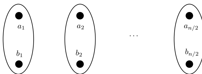
■ Figure 3 Union of (2,2)-thresholds.
