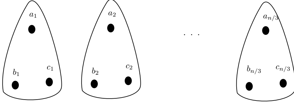
■ Figure 2 The Moon-Moser access structure.
